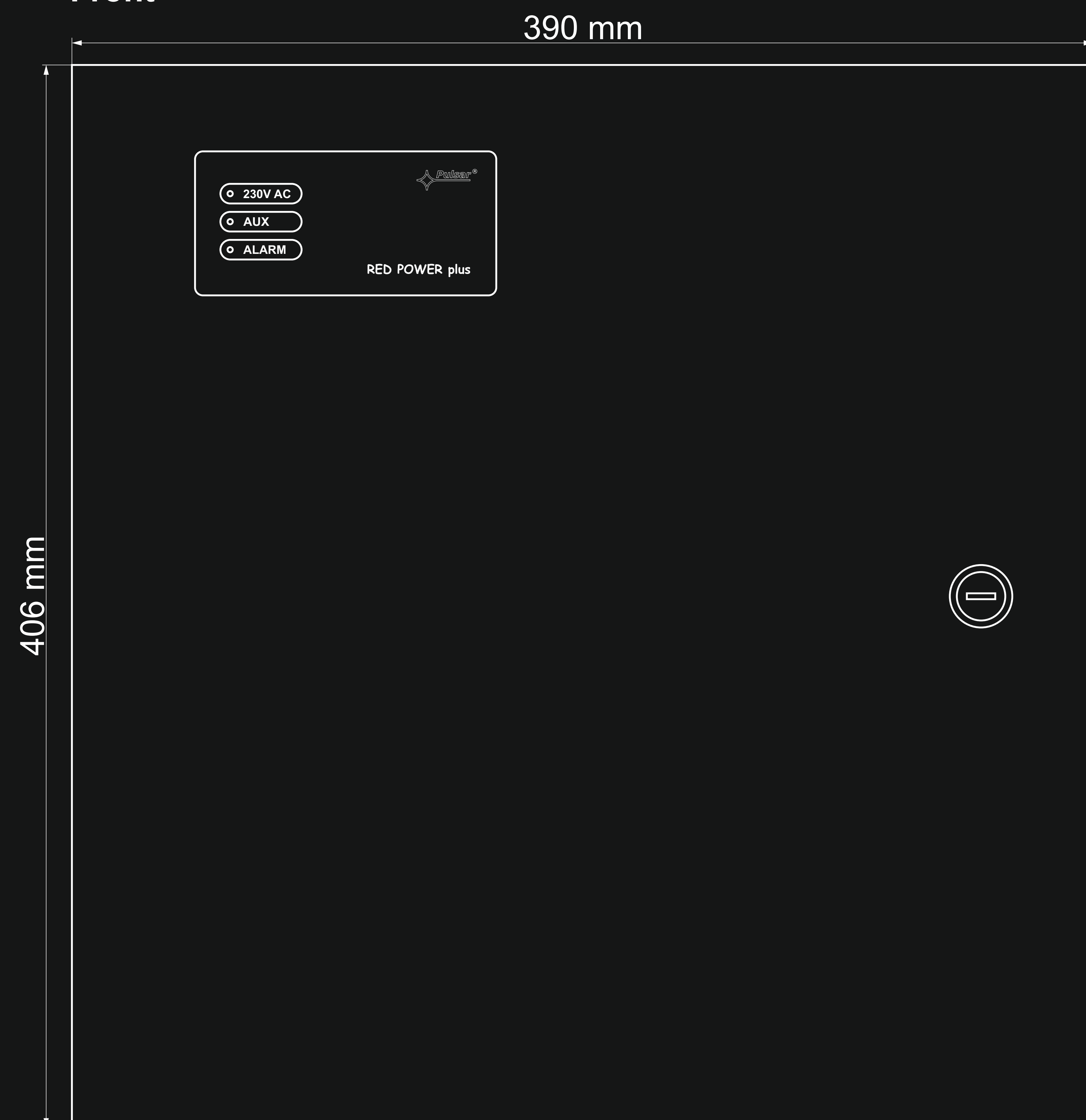
Front
