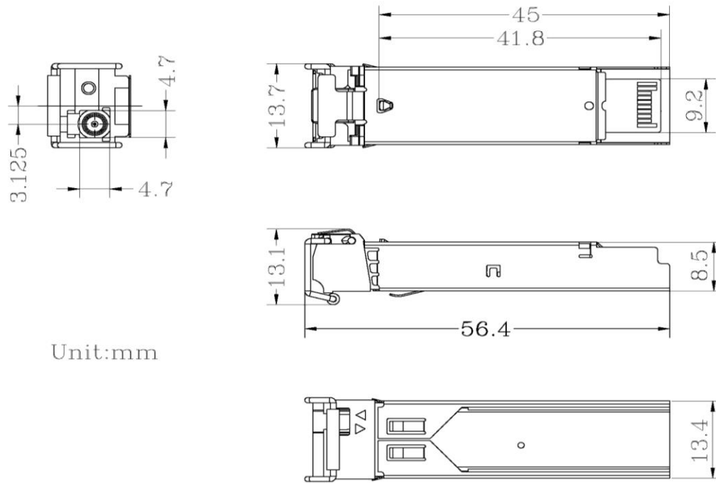
Figure 5. Outline Drawing
